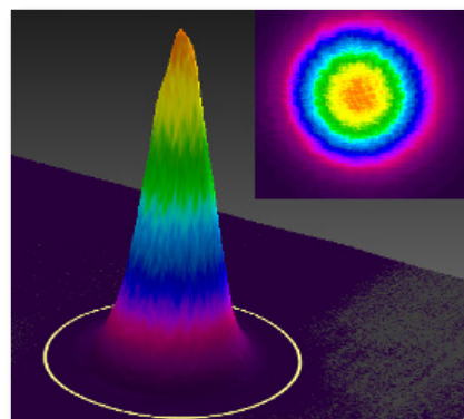
Typical TEM 00 Beam Profile
